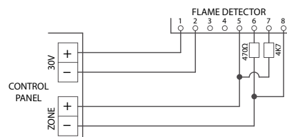
Wiring diagram
